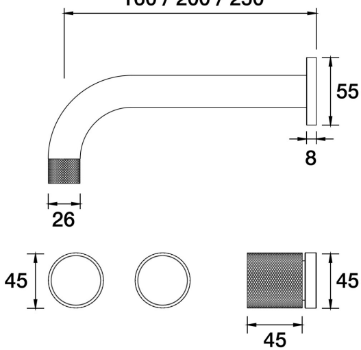
IDK Marble Wall Bath Set 200mm Outlet Nero IDK012.2.43 - Brass
