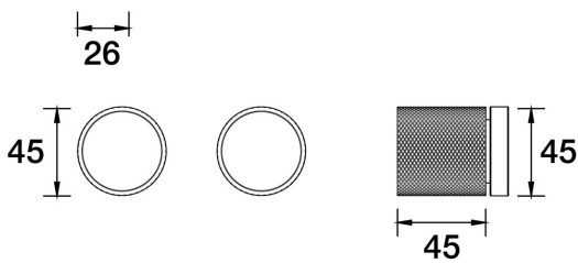
IDK Marble Wall Bath Set 200mm Outlet Nero Marquina 89,012.2.68 - Autumn Bronze
