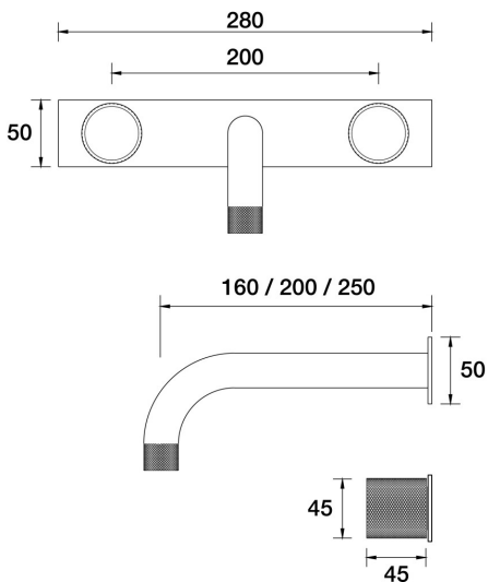
IDK Marble Wall Bath Set 200mm Outlet Nero Marble on Plate B39.022.4.75 - Forest Mist
