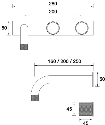
IDK Marble Wall Bath Set 200mm Outlet Nero Marble on Plate - Offset B39.022.6.27 - Satin Pearl
