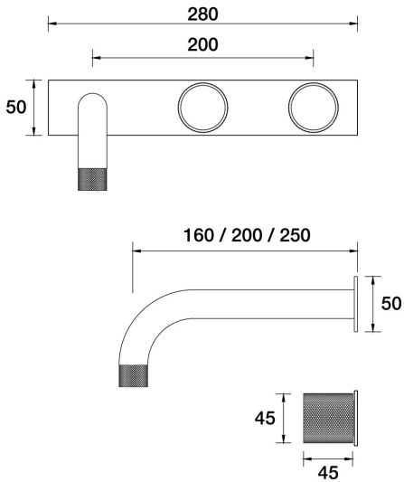
IDK Marble Wall Bath Set 200mm Outlet Nero Marble on Plate - Offset B39.022.6.32 - Midnight Black
