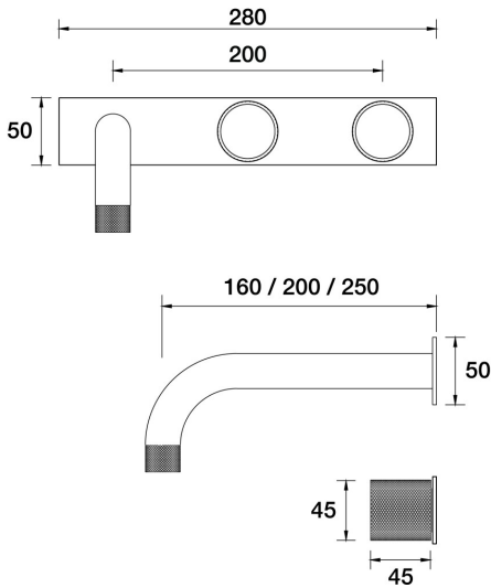
IDK Marble Wall Bath Set 200mm Outlet Nero Marble on Plate - Offset B39.022.6.44 - Antique Copper
