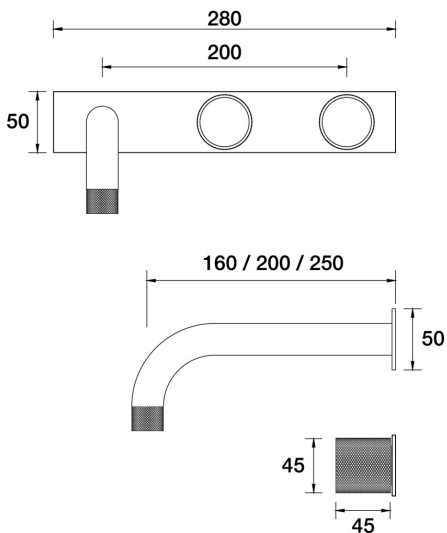
IDK Marble Wall Bath Set 200mm Outlet Nero Marble on Plate - Offset B39.022.6.54 - Volcanic Grey
