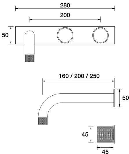
IDK Marble Wall Bath Set 200mm Outlet Nero Marble on Plate - Offset B39.022.6.75 - Forest Mist
