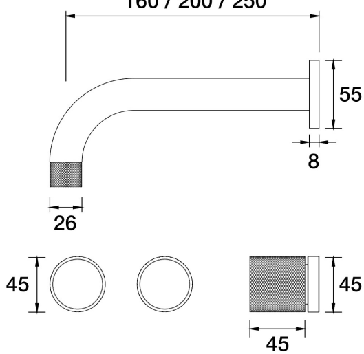
IDK Marble Wall Bath Set 250mm Outlet Nero Marble 89.023.2.27 - Satin Pearl
