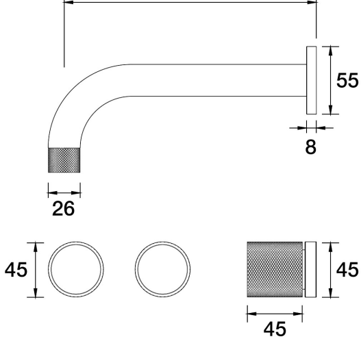
IDK Marble Wall Bath Set 250mm Outlet Nero Marble 809.023.2.40 - Rumbled Brass
