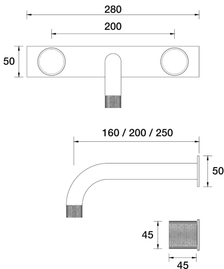
IDK Marble Wall Bath Set 250mm Outlet Bianco Marble on Plate B39.023.3.45 - Native Brass
