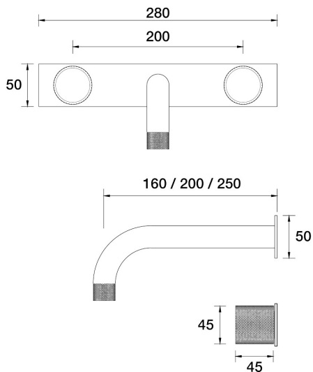
IDK Marble Wall Bath Set 250mm Outlet Nero Marble on Plate B39.023.4.01 - Chrome
