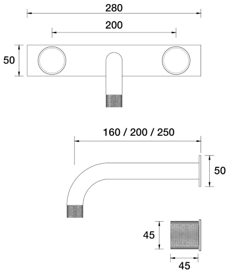
IDK Marble Wall Bath Set 250mm Outlet Nero Marble on Plate B39.023.4.26 - Black Sapphire
