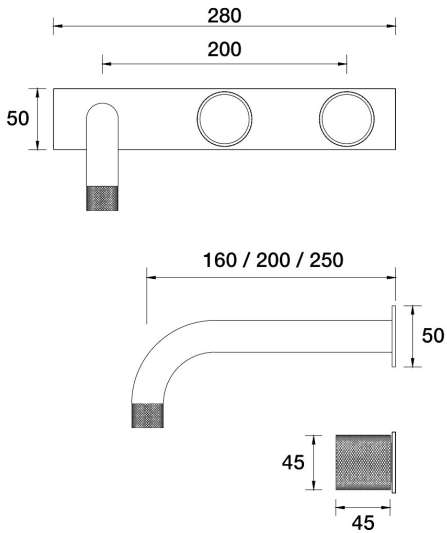
IDK Marble Wall Bath Set 250mm Outlet Bianco Marble on Plate - Offset B39.023.5.54 - Volcanic Grey
