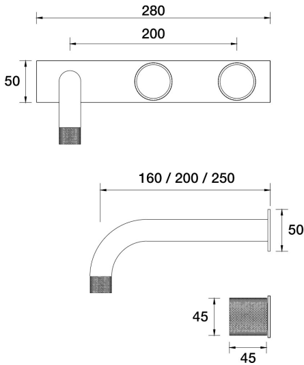
IDK Marble Wall Bath Set 250mm Outlet Nero Marble on Plate - Offset B39.023.6.44 - Antique Copper
