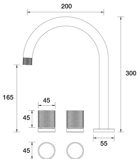
IDK Marble Sink Set Hob Swivel Nero Marble B39.051.2.48 - Copper
