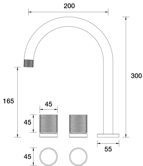
IDK Marble Sink Set Hob Swivel Nero Marble B39.051.2.52 - Burnished
