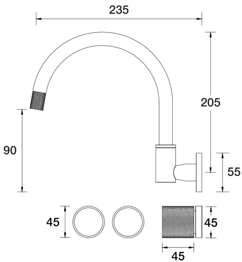
IDK Marble Sink Set Wall Swivel Nero Marble B39.052.2.32 - Midnight Black
