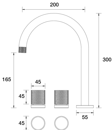
IDK Marble Spa Set Hob Swivel Nero Marble B39.061.2.21 - Brushed Rose Gold
