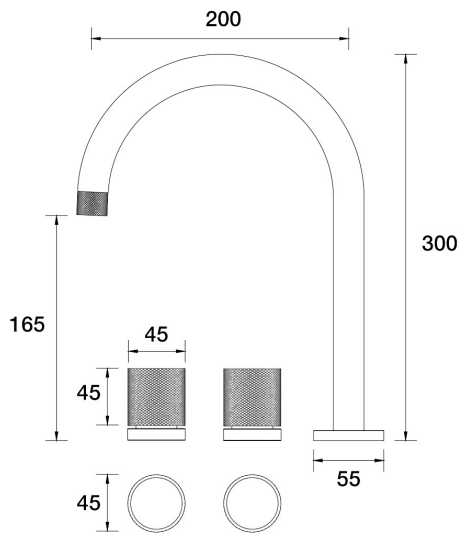
IDK Marble Spa Set Hob Swivel Nero Marble B39.061.2.39 - Antique Bronze
