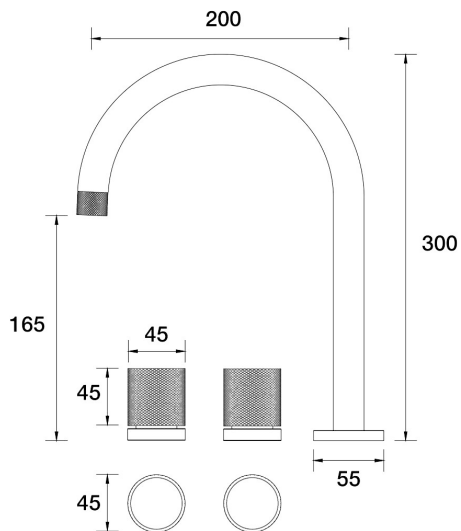
IDK Marble Spa Set Hob Swivel Nero Marble B39.061.2.42 - Brushed Copper
