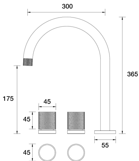
IDK Marble Spa Set XL Hob Swivel Bianco Marble B39.063.1.21 - Brushed Rose Gold
