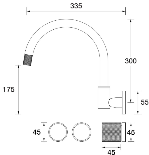
IDK Marble Spa Set XL Wall Swivel Nero Marble B39.064.2.47 - Luminick
