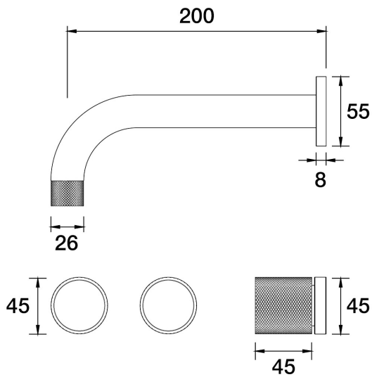
IDK Marble Wall Basin Set 200mm Outlet Bianco Marble B39.152.1.48 - Copper
