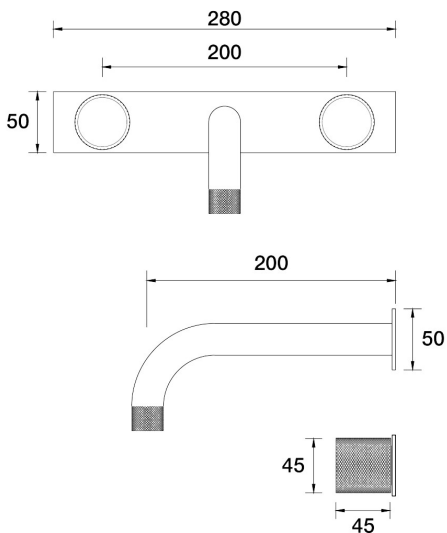
IDK Marble Wall Basin Set 200mm Outlet Bianco Marble on Plate B39.152.3.52 - Burnished
