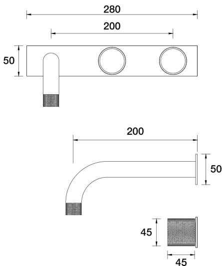
IDK Marble Wall Basin Set 200mm Outlet Bianco Marble on Plate - Offset B39.152.5.70 - Sea Spray
