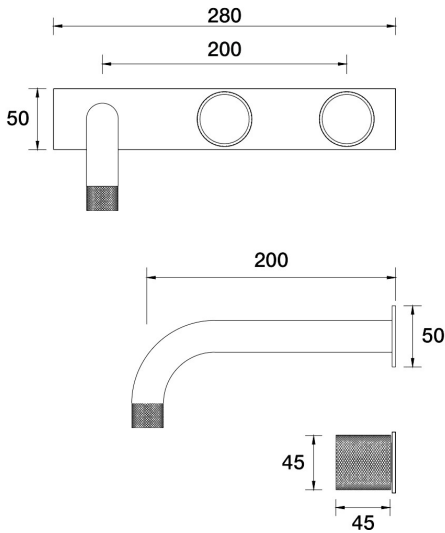
IDK Marble Wall Basin Set 200mm Outlet Nero Marble on Plate - Offset B39.152.6.25 - Brushed Nickel
