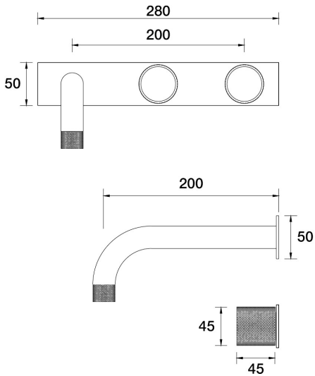
IDK Marble Wall Basin Set 200mm Outlet Nero Marble on Plate - Offset B39.152.6.42 - Brushed Copper
