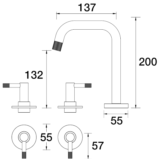
Elm Basin Set Swivel B40.011.1.01 - Chrome
