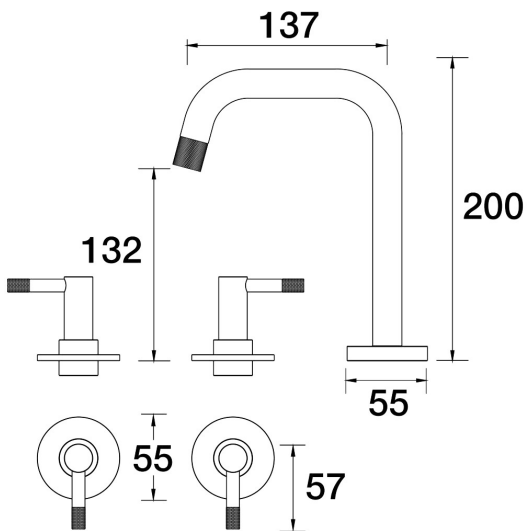
Elm Basin Set Swivel B40.011.1.34 - Matt Black
