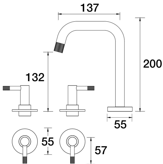
Elm Basin Set Swivel B40.011.1.57 - Matt Nickel
