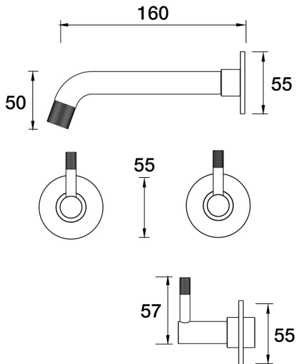
Elm Wall Bath Set 160mm Outlet B40.021.1.40 - Rumbled Brass
