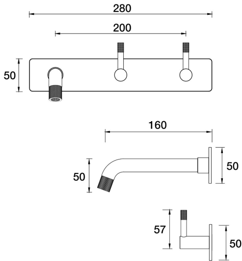
Elm Wall Bath Set 160mm Outlet On Plate - Offset B40.021.3.32 - Midnight Black
