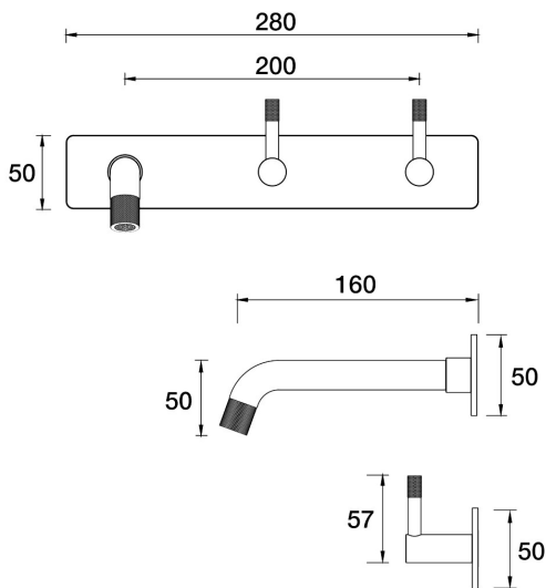
Elm Wall Bath Set 160mm Outlet On Plate - Offset B40.021.3.40 - Rumbled Brass
