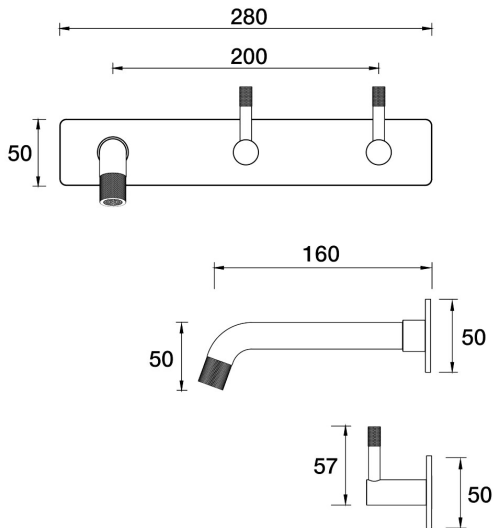
Elm Wall Bath Set 160mm Outlet On Plate - Offset B40.021.3.45 - Native Brass
