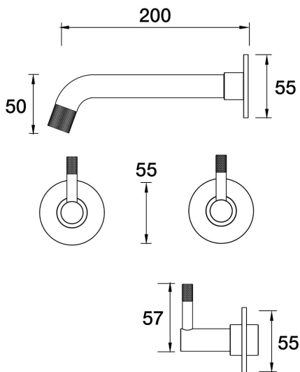
Elm Wall Bath Set 200mm Outlet B40.022.1.12 - 23k Brushed Gold
