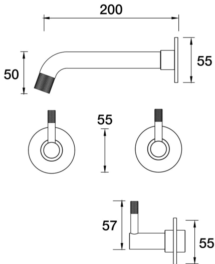
Elm Wall Bath Set 200mm Outlet B40.022.1.43 - Brass
