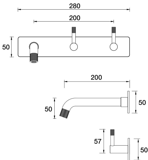
Elm Wall Bath Set 200mm Outlet On Plate - Offset B40.022.3.39 - Antique Bronze
