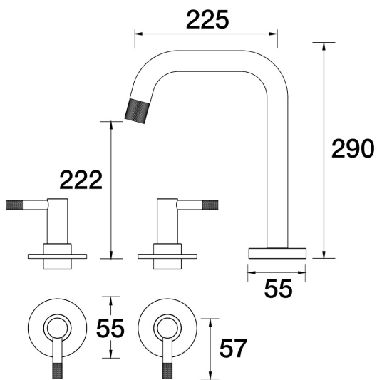
Elm Spa Set Hob Swivel B40.061.1.27 - Satin Pearl
