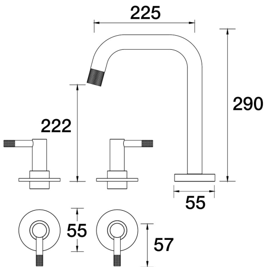
Elm Spa Set Hob Swivel B40.061.1.34 - Matt Black
