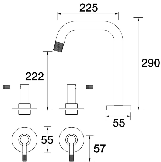
Elm Spa Set Hob Swivel B40.061.1.44 - Antique Copper
