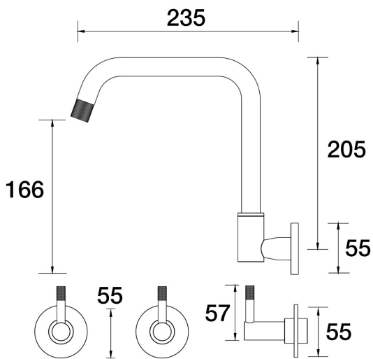
Elm Spa Set Wall Swivel B40.062.1.47 - Luminick
