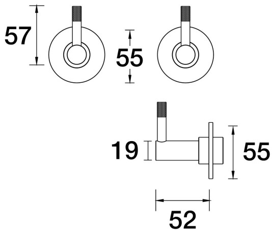
Elm Top Assemblies Wall Pair B40.082.1.43 - Brass
