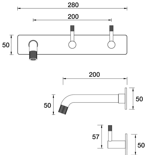
Elm Wall Basin Set 200mm Outlet On Plate - Offset B40.152.3.26 - Black Sapphire
