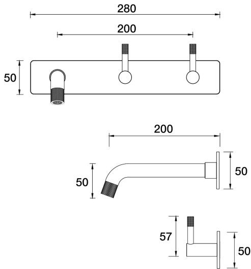
Elm Wall Basin Set 200mm Outlet On Plate - Offset B40.152.3.48 - Copper
