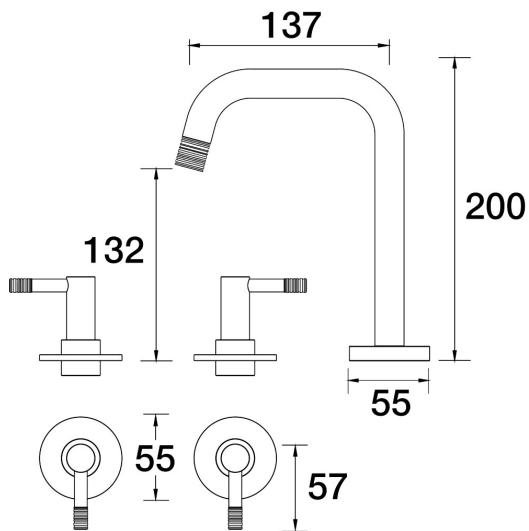
Elm Lane Basin Set Swivel B42.011.1.68 - Autumn Bronze
