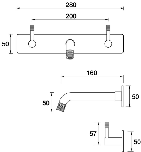
Elm Lane Wall Bath Set 160mm Outlet On Plate B42.021.2.01 - Chrome
