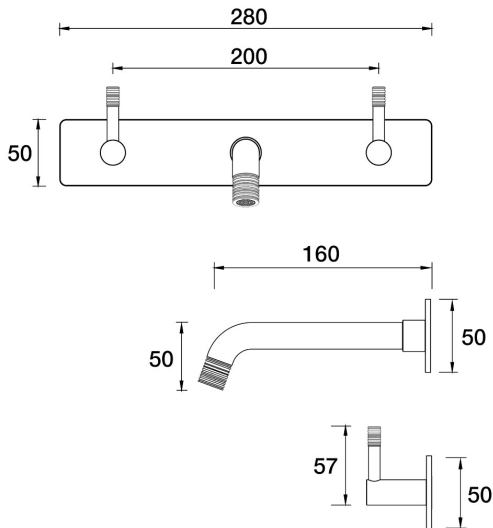
Elm Lane Wall Bath Set 160mm Outlet On Plate B42.021.2.26 - Black Sapphire
