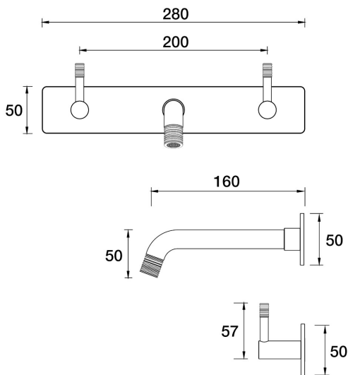
Elm Lane Wall Bath Set 160mm Outlet On Plate B42.021.2.39 - Antique Bronze
