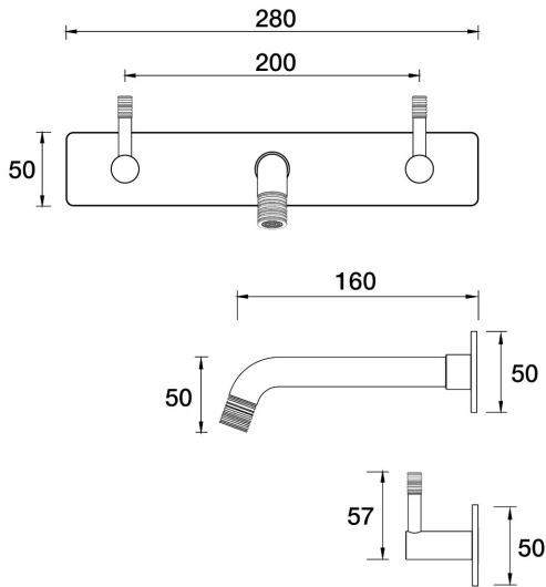
Elm Lane Wall Bath Set 160mm Outlet On Plate B42.021.2.57 - Matt Nickel
